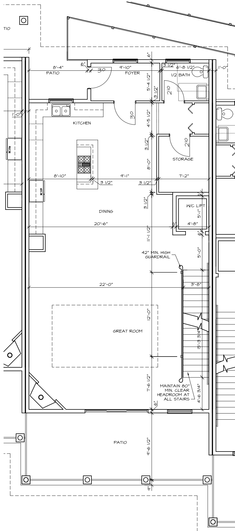
TYP. "B" TYPE UNIT FIRST FLOOR PLAN
